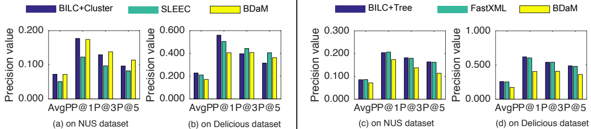
Figure 4: Comparison of two acceleration methods of BILC. Figures (a) and (b) show comparisons among BILC+Cluster and SLEEC with the same clusters, while figures (c) and (d) show comparisons between BILC+Tree and FastXML with the same decision tree growing method. To judge the performance of acceleration methods of BILC, we also compared them with BDaM.
