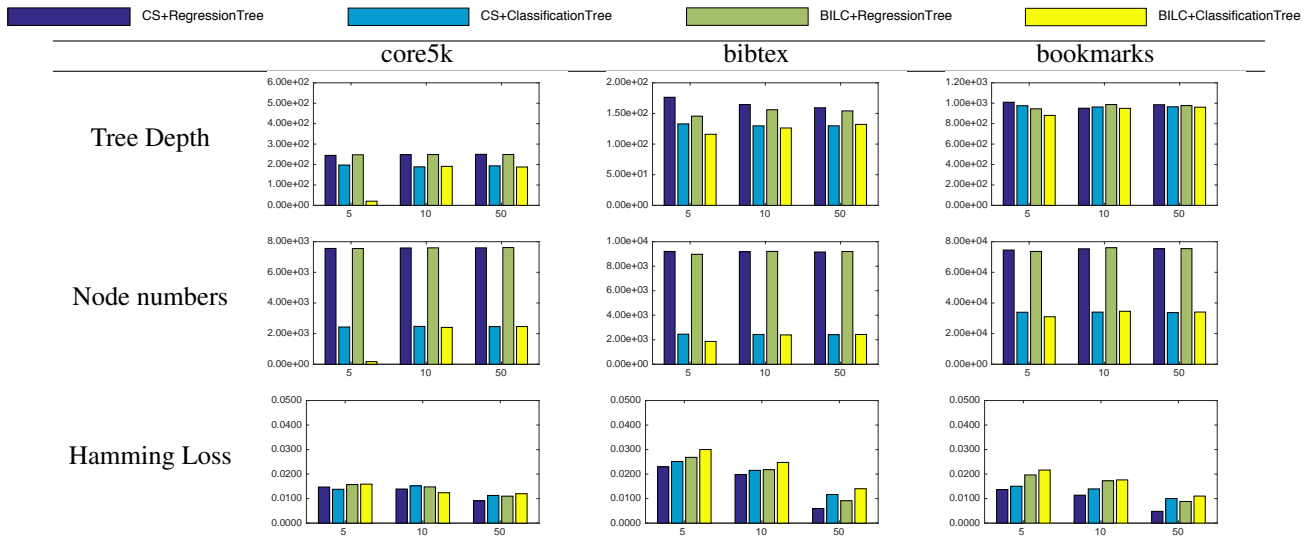
Figure 1: Comparison between classification and regression. The x-axis in each figure denotes the embedding dimension.
