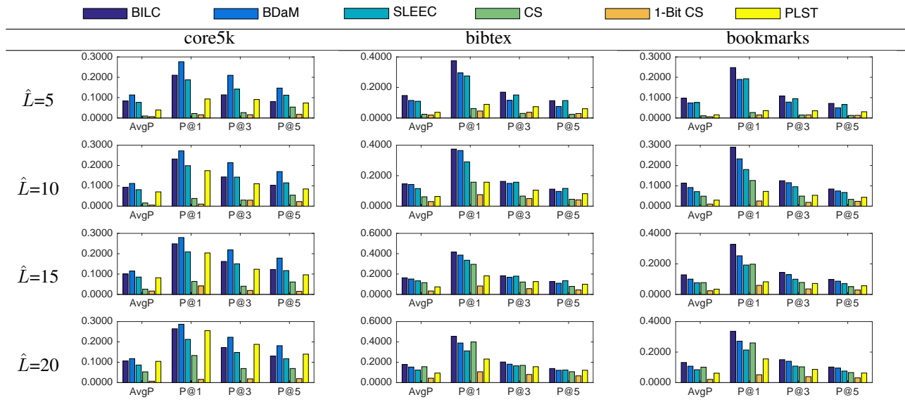
Figure 3: Comparison among different embedding-based multi-label classification methods on three datasets and four embedding dimensions.
