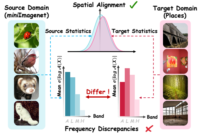
Figure 1: While spatial alignment is achieved, frequency discrepancies persist. “A”, “L”, “M”, and “H” denote All-, Low-, Middle-, and High-Frequency Bands, respectively.
