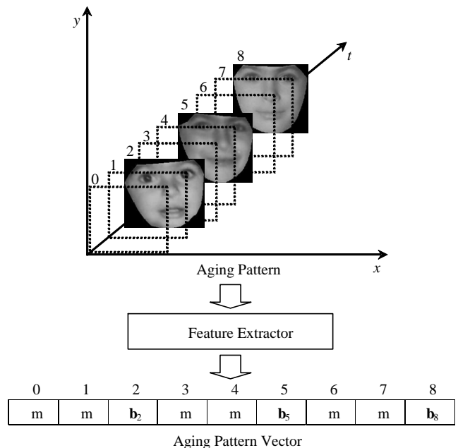
Figure 1: Vectorization of the aging pattern. The ages (0-8) are marked at the top-left to the corresponding positions and above the corresponding feature vectors. The missing parts in the aging pattern vector are marked by ‘m’.
